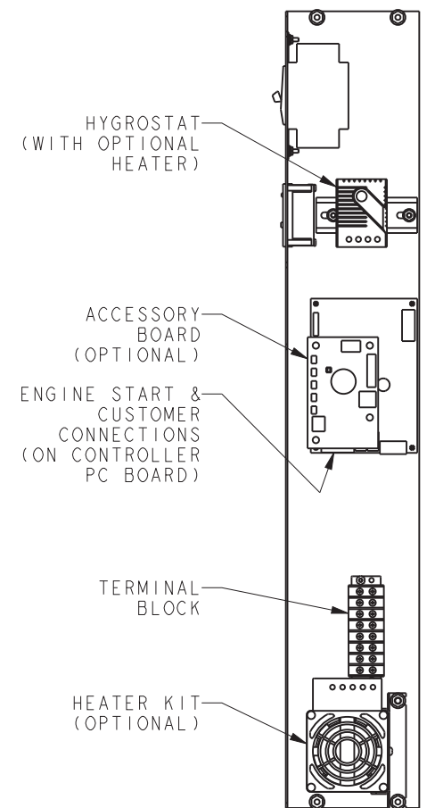
VIEW C
