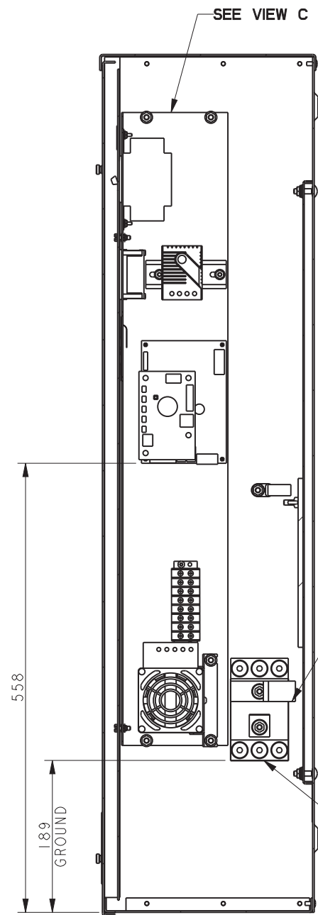
SECTION B-B
