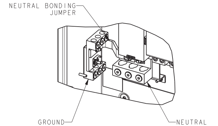
VIEW D
