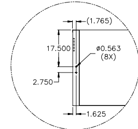
STEP HOLE DETAIL
